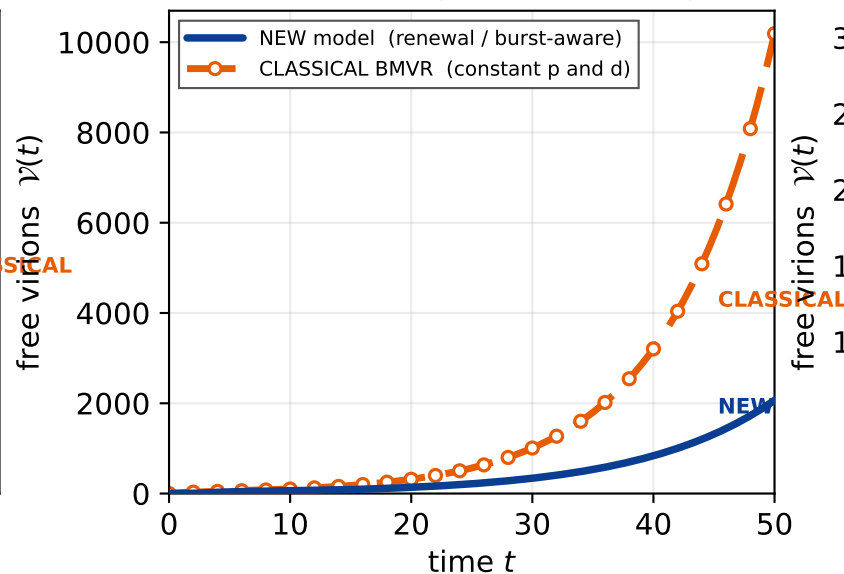
(b) supercritical, \mu > 0 \beta = 1.0, \mu = 0.2, \delta = 0.05 \mid \gamma T = 0.03, c = 0.2 \mid R_0 = 2.10
