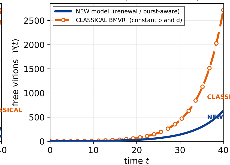
(f) free-virion seed only ( I_0 = 0 ) \beta = 1.0, \mu = 0.0, \delta = 0.1 \mid \gamma T = 0.05, c = 0.2 \mid R_0 = 2.7
