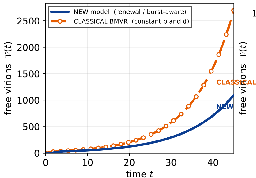
(a) supercritical, \mu = 0 \beta = 1.0, \mu = 0.0, \delta = 0.1 \mid \gamma T = 0.04, c = 0.25 \mid R_0 = 1.76
