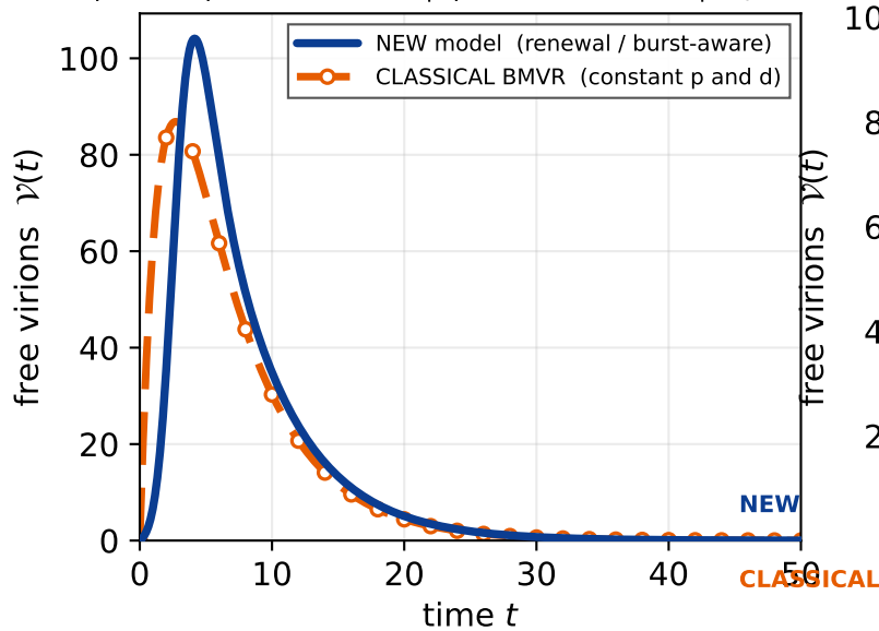
(d) subcritical R_0 < 1 \beta = 1.0, \mu = 0.0, \delta = 0.1 \mid \gamma T = 0.01, c = 0.4 \mid R_0 = 0.27
