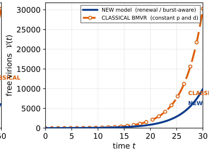
(c) fast burst (large \delta ) \beta = 1.0, \mu = 0.0, \delta = 0.5 \mid \gamma T = 0.25, c = 0.3 \mid R_0 = 2.5
