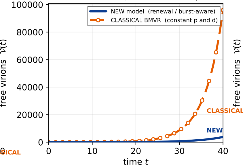
(e) high intracellular death \beta = 1.0, \mu = 0.9, \delta = 0.1 \mid \gamma T = 0.5, c = 0.25 \mid R_0 = 2.63
